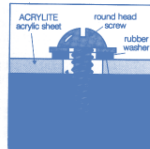
Details for bolting small sheet to a frame.
