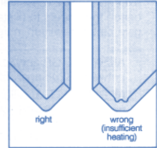
Correct and incorrect bends.
