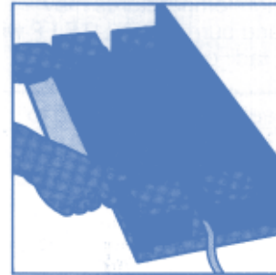
Heating acrylic sheet with a strip heater.
