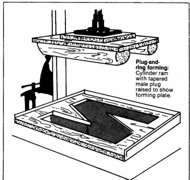
Plug-and-ring forming: Male plug.
