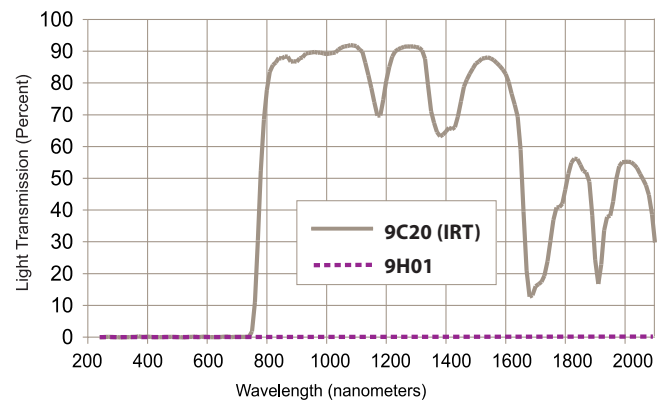
Transmission of ACRYLITE® GP sheet, Color # 9C20 (IRT) and # 9H01
